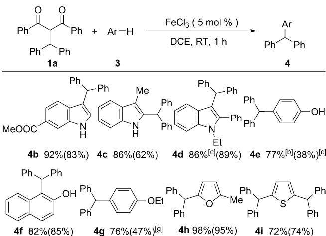
Scheme 3. The reaction of 1a with aromatic compounds 3 . Reaction conditions: 1a (0.2 mmol), 3 (0.2 mmol), FeCl 3 (5 mol %), DCE (5.0 mL), RT, 1 h. Yield for when diphenylmethanol was used instead of 1a . The yield in parentheses for when 4 was used. [a] FeCl 3 (10 mol %), 50 °C, 24 h. [b] 2,4-Dialkylation product 4e' was obtained in 5% yield. [c] 4e' was obtained in 38% yield. [d] 2,4-Dialkylation product 4g' was obtained in 46% yield.
